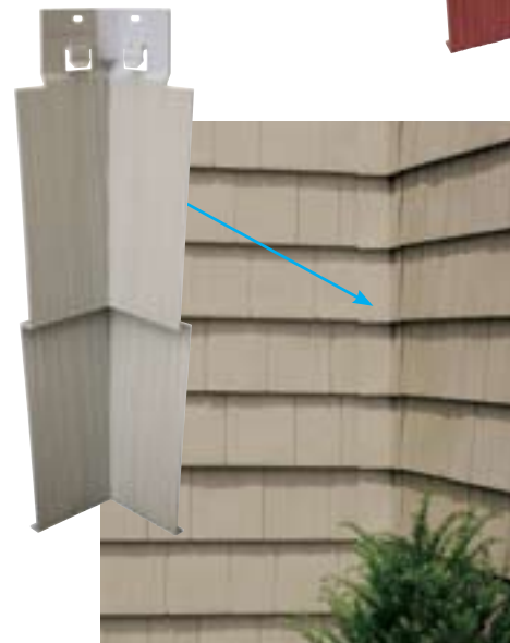
Double 7" mitered inside cornerpost.
